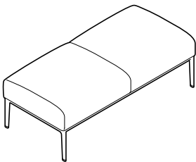
864/3 ☐44 ☐144 ☐69 (☐17 3 / 8 " ☐56 3 / 4 " ☐27 1 / 8 " )
