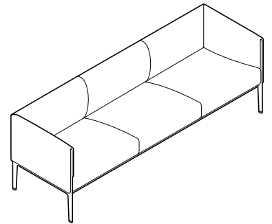
863/5 ☐44 ☐72 ☐218 ☐69 (☐17 3 / 8 " ☐28 3 / 8 " ☐85 7 / 8 " ☐27 1 / 8 " )
