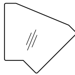
541/10 Connecting leaf 45° 75 x 15 x 75 x 15 x 75 x 24 x 24 (29½" x 5⅞" x 29½" x 5⅞" x 29½" x 9½" x 9½")
