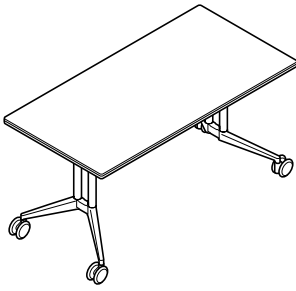
621/5 , 75x150 (29½" x 59"), with castors 621/1 , 75x150 (29½" x 59"), with glides 621/3 , 75x225 (29½" x 88⅝"), with glides
