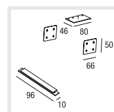
CANYON 100 Linienverbinder CANYON 100 Linear connector CANYON 100 Giunto lineare
