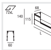
CANYON 60 Installation channel
