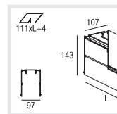
CANYON 100 Installation channel
