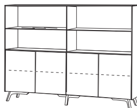
DR8222 L198 P47 H130,1
